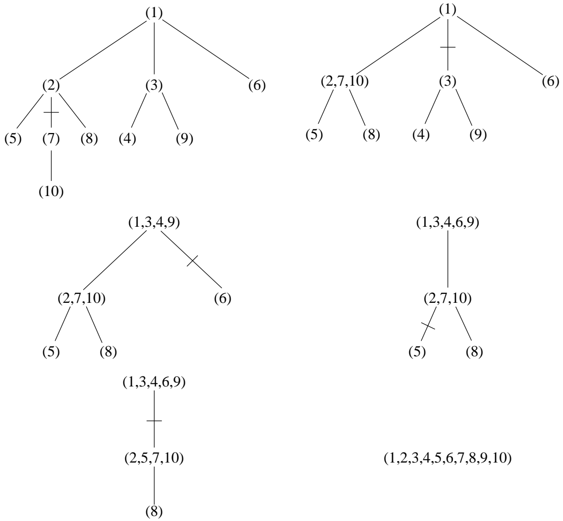
Figure 2: The cutting procedure for a random recursive tree on [10] , with the cuts indicated.
