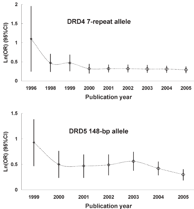
Figure 3. Cumulative syntheses of studies for the DRD4 7-repeat allele and the DRD5 148-bp alleles shown by overall \ln(\text{OR}) , the 4-, 5-repeat alleles and DAT1 480-bp allele (data not shown) were similar with the 7-repeat allele.
