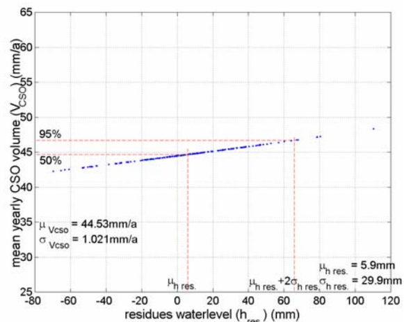
Figure 8 Influence of uncertainties in outcomes of calibrated model on probability distribution of CSO volume.
