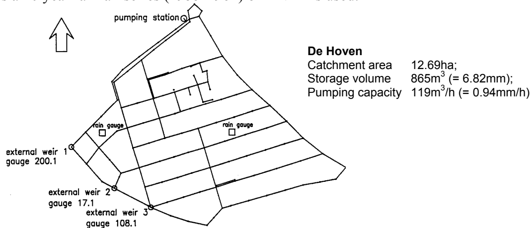
Figure 4 Layout sewer system 'De Hoven' (from: Clemens, 2001).
