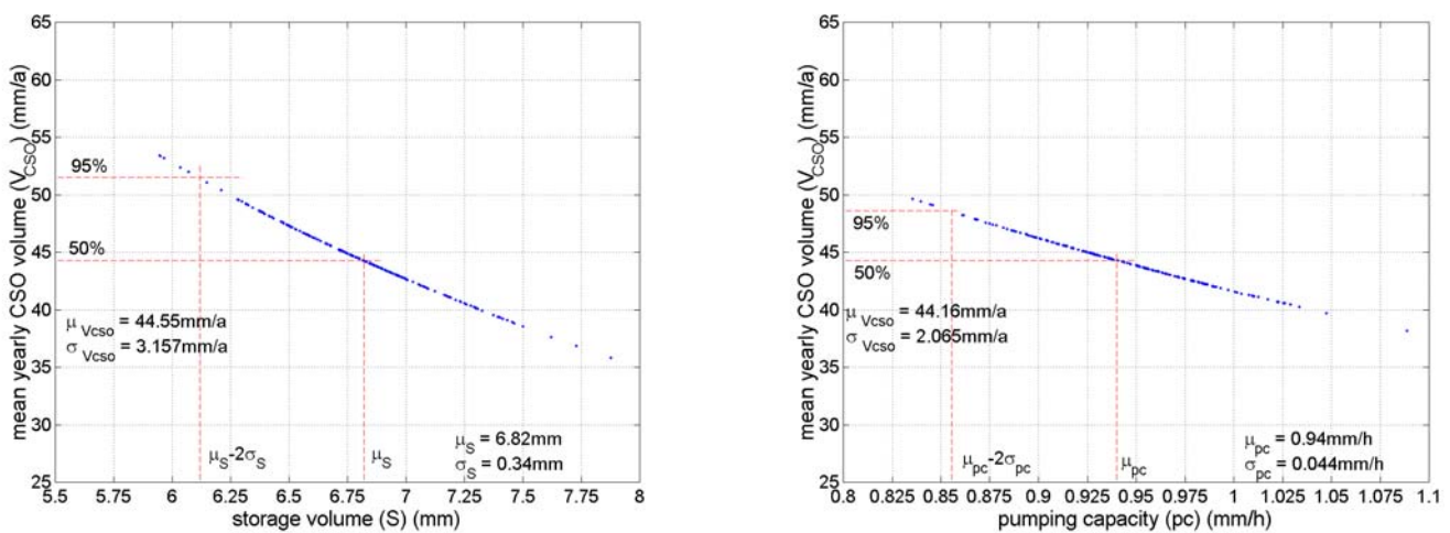
Figure 6 Influence of uncertainties in dimensions on probability distribution of CSO volume.
