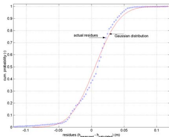
Figure 7 Probability distribution for the residues obtained after calibration of the hydrodynamic model (adapted from: Clemens, 2001). These results are used as input of the Monte Carlo simulation with the reservoir model.
