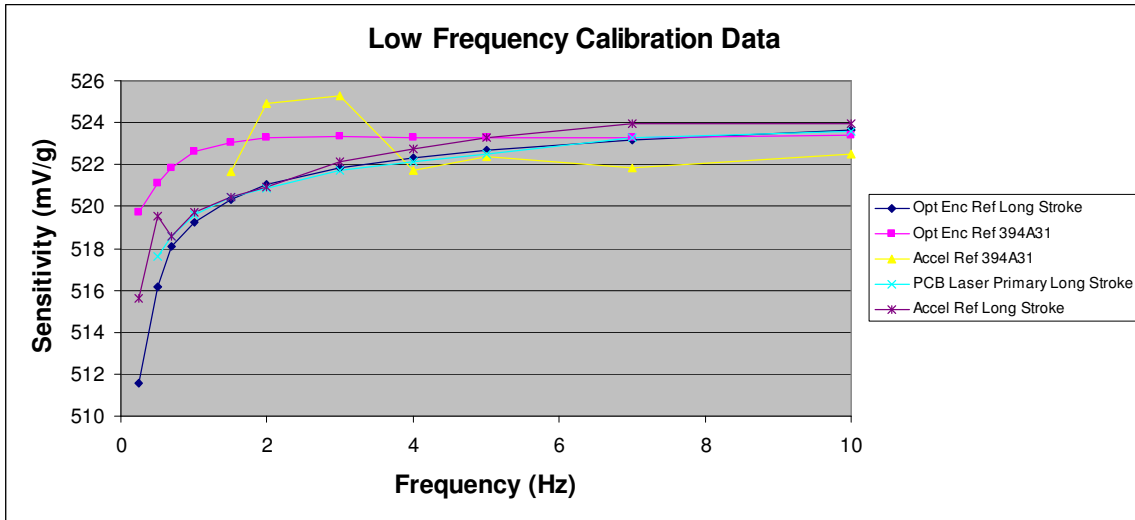
Figure 9. Calibration results for different system configurations from 0.25 Hz to 10 Hz
