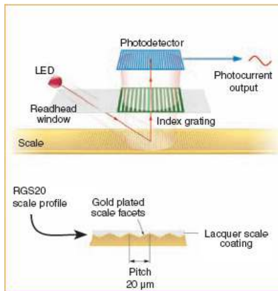
Figure 7. Optical Encoder Operation (graphic courtesy Renishaw)
