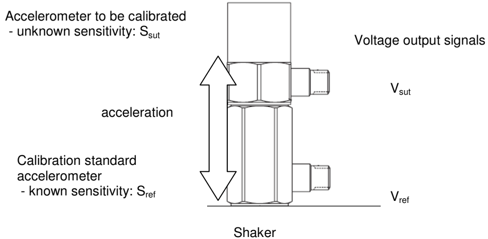
Figure 1: Back-to-back technique.
