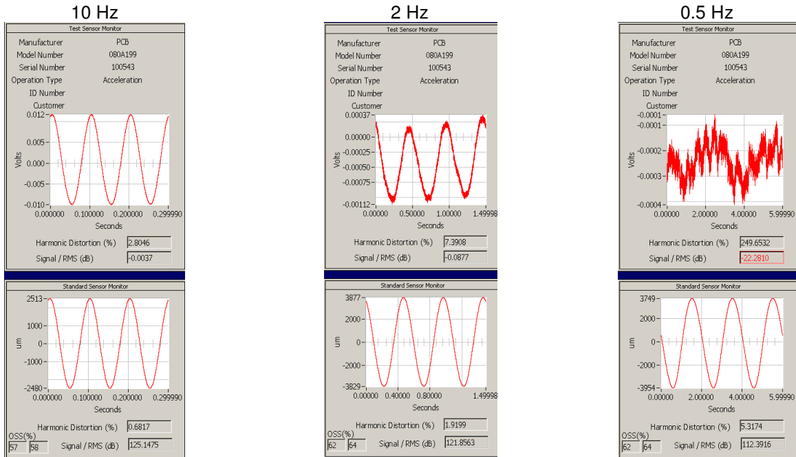
Figure 8. Reference sensor measurement signals from accelerometer (upper plot) and optical encoder (lower plot), displayed at 10 Hz, 2 Hz and 0.5 Hz as indicated
