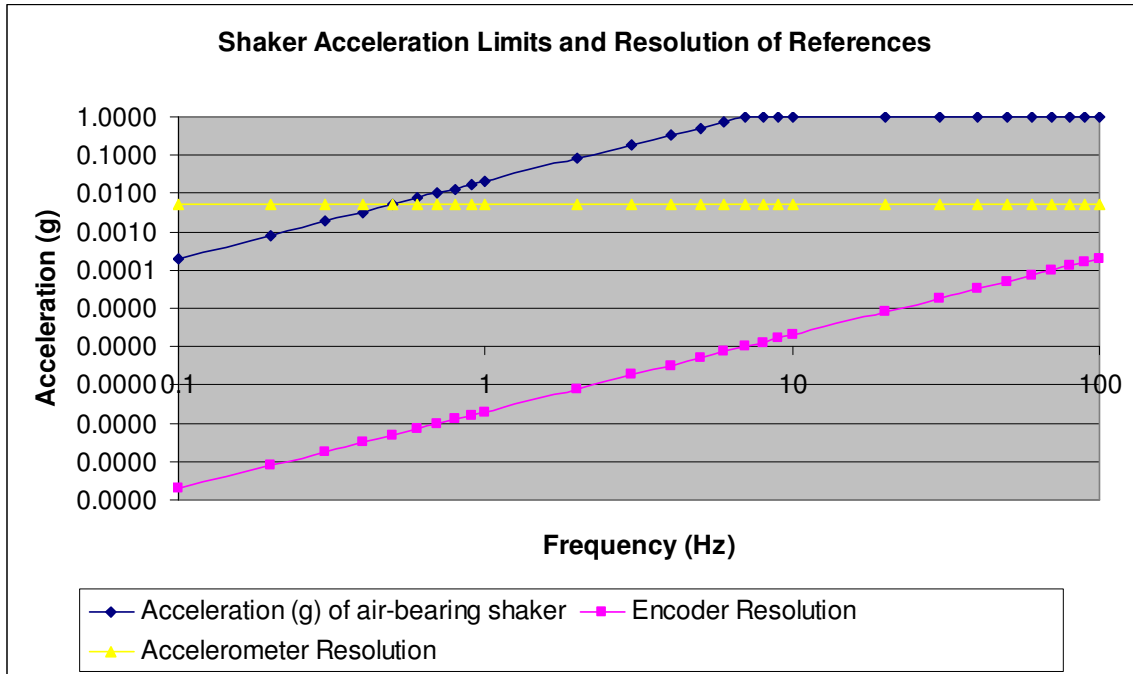
Figure 5. Theoretical limits of accelerometer* and optical encoder reference sensors charted against air-bearing shaker acceleration limits due to maximum stroke. *Accelerometer resolution displayed is based upon the manufacturer's broadband RMS resolution.
