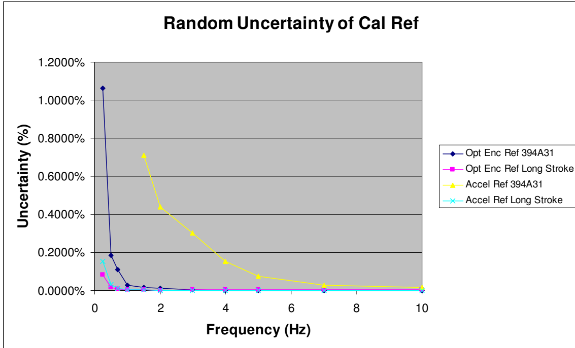
Figure 10. Random Uncertainties using PCB Q353B51 accelerometer on both 394A31 air-bearing and long stroke shakers
