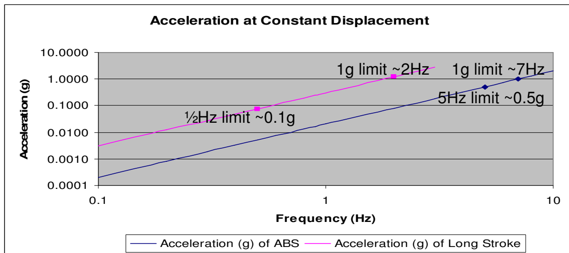
Figure 4: Maximum theoretical acceleration limits for the 10 mm stroke air-bearing shaker (ABS) and the 6 in. long stroke shaker
