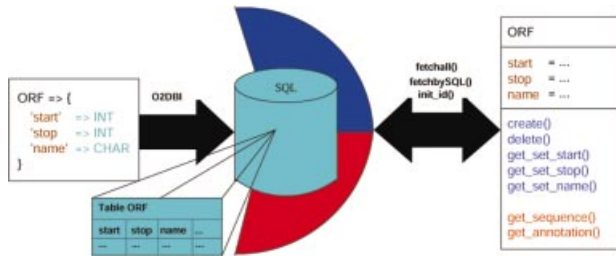
Figure 3. O2DBI maps Perl objects to relational tables, generating both SQL tables and Perl modules.
