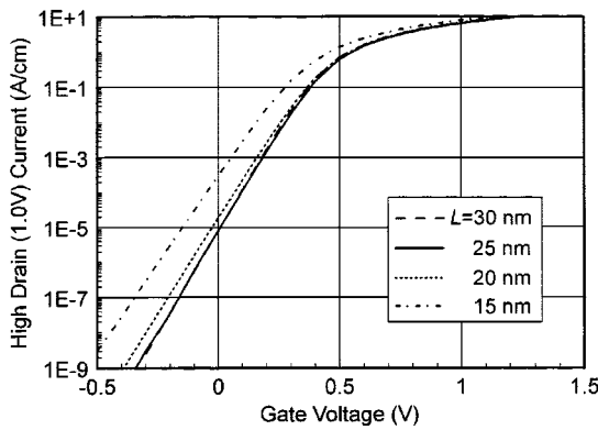
Fig. 16. Subthreshold currents for channel lengths from 30 to 15 nm. I_{off} = 10^{-5} \text{ A/cm} ( 1 \text{ nA}/\mu\text{m} ) for 20, 25, and 30 nm devices. From [27].
