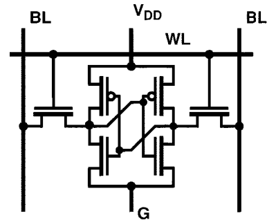
Fig. 26. Six transistor Static RAM cell. Cell is addressed by the wordline (WL) and the data is read out via the bit line pair (BL). Inset shows a set of superimposed transfer curves for the two halves of the SRAM cell showing how the noise immunity (shaded box) is affected by a threshold voltage shift in one of the halves.
