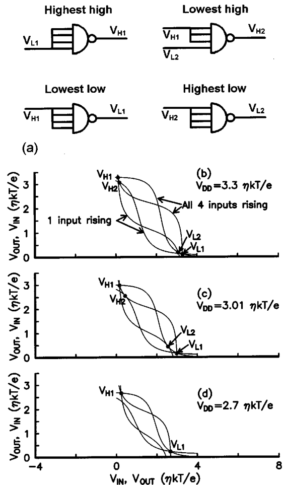
Fig. 10. Illustration of minimum swing determination using ideal four-input CMOS NAND gates. (a) Set of schematics defining conditions for best- and worst case logic outputs. (b)–(d) Transfer characteristics in the form of "eye" diagrams. Output voltage versus input voltage and input voltage versus output voltage for the cases when only one input is switching and when all four inputs are switching. Inputs that are not switching are held at V_{H1} . (b) Logic swing is above the minimum. Self-consistent low output states are between V_{L1} and V_{L2} and self-consistent high output states are between V_{H1} and V_{H2} . (c) Logic swing is exactly at minimum. (d) Logic swing is below the minimum; there are no fully self-consistent output logic states.
