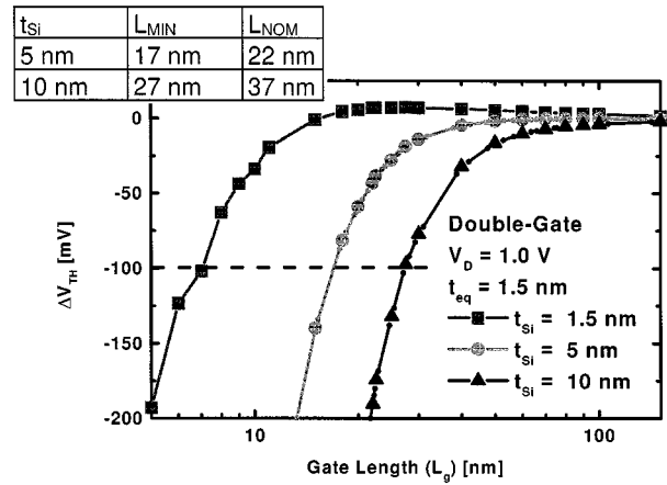
Fig. 19. Threshold voltage rolloff for DG-FET with equivalent gate oxide thickness ( t_{eq} ) of 1.5 nm and silicon channel thickness t_{Si} of 1.5, 5, and 10 nm. 1.5-nm thickness is not practical and is included here only as a reference. DIBL is taken into consideration by plotting the threshold voltage rolloff at a drain voltage V_D equal to the power supply voltage.
