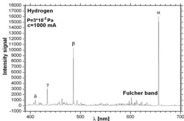
Fig.7 The emission spectrum measured in hydrogen plasma.
