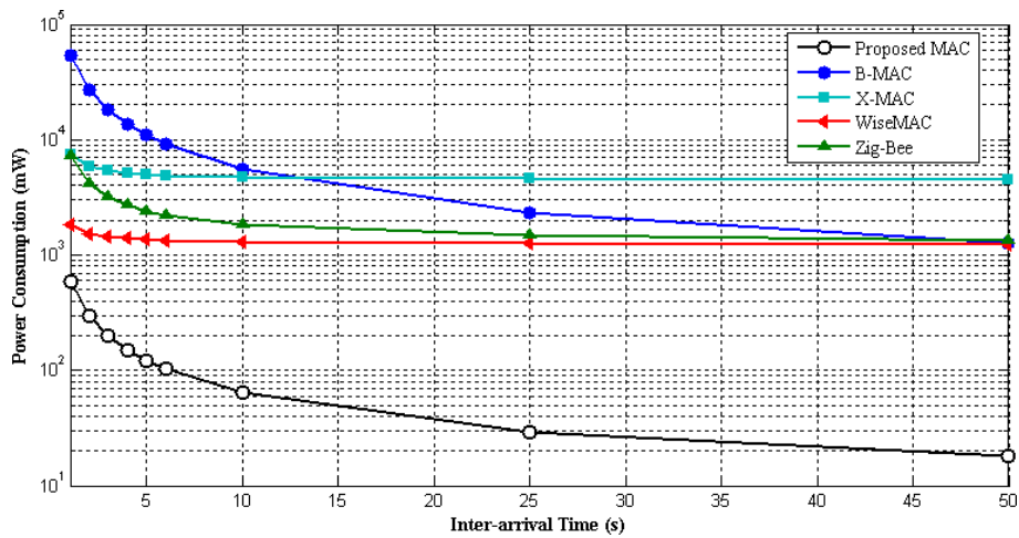
Figure 16 Power consumption.
