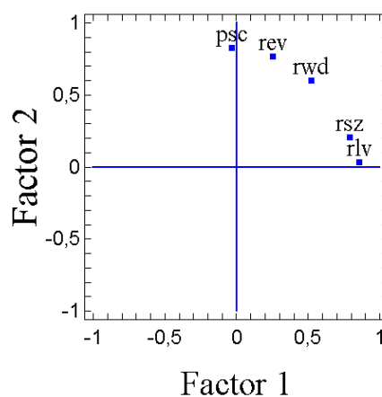
Fig. 13: Factor loadings of room attributes only. Two factors extracted. Rotation: Varimax.
