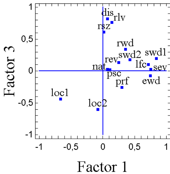
11, 12: Plots of factor loadings on the three extracted factors. Rotation: Varimax
