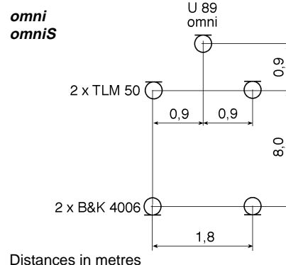
Fig. 1: Microphone set-ups for recording of stimuli.
