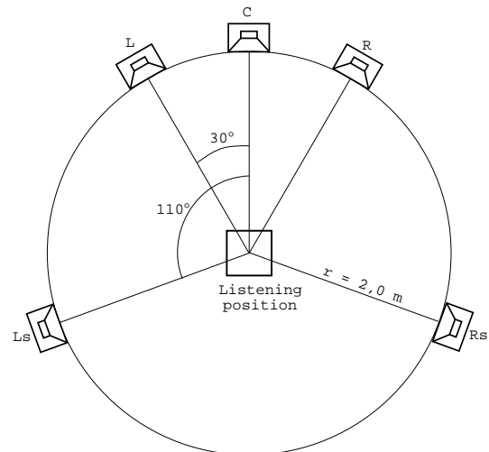
Fig. 3. Loudspeaker set-up
