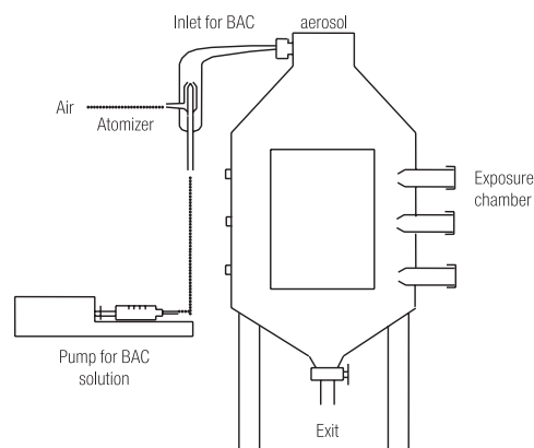
Fig. 2. Technical scheme of nose-only inhalation exposure conditions for toxicity testing of BAC aerosol.
