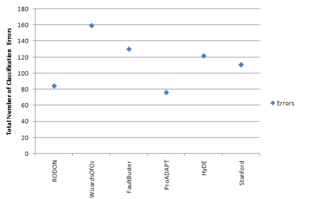
Fig. 7. Industrial track tier 2 classification errors by DA
