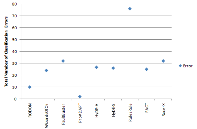
Fig. 3. Industrial track tier 1 classification errors by DA
