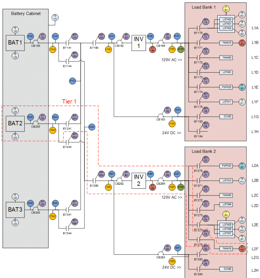
Fig. 1. The ADAPT EPS (Electrical Power System)
