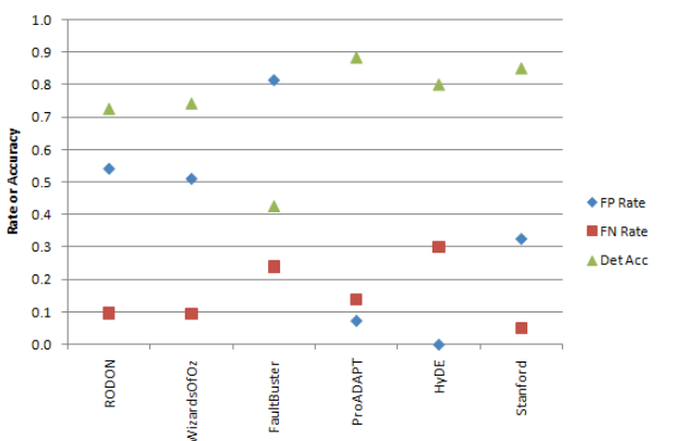
Fig. 6. Industrial track tier 2 false positive rate, false negative rate, and detection accuracy by DA
