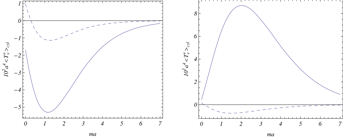
Figure 3: Boundary induced parts in the VEVs of the energy density, a^4\langle T_0^0 \rangle_{\text{cyl}} (full curves), and radial stress, a^4\langle T_1^1 \rangle_{\text{cyl}} (dashed curves), as functions of the parameter ma for q = 2 . The left panel corresponds to the interior region with r/a = 0.5 and the right panel corresponds to the exterior region with r/a = 1.5 .
