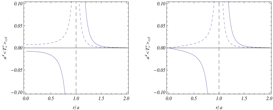
Figure 1: Boundary induced parts in the VEVs of the energy density, a^4 \langle T_0^0 \rangle_{\text{cyl}} (full curves), and radial stress, a^4 \langle T_1^1 \rangle_{\text{cyl}} (dashed curves), for a massless fermionic field as functions of the radial coordinate. The left panel is plotted for q = 1 (Minkowski spacetime) and for the right panel q = 2 .
