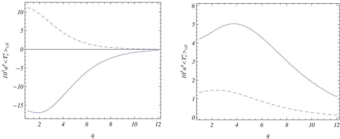
Figure 2: Boundary induced parts in the VEVs of the energy density, a^4 \langle T_0^0 \rangle_{\text{cyl}} (full curves), and radial stress, a^4 \langle T_1^1 \rangle_{\text{cyl}} (dashed curves), for a massless fermionic field as functions of the parameter q . The left panel corresponds to the interior region with r/a = 0.5 and the right panel corresponds to the exterior region with r/a = 1.5 .
