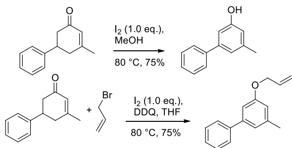
Scheme 18. \alpha,\beta -unsaturated cyclohexane to phenol using molecular I 2 /DDQ.
