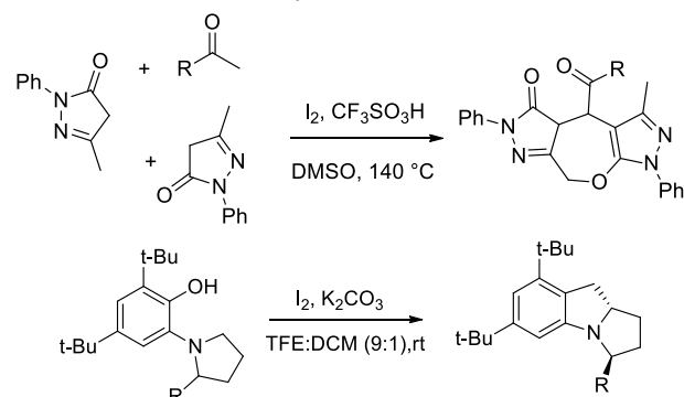
Scheme 23. Regioselective oxidation and formation of N,O-Acetals.
