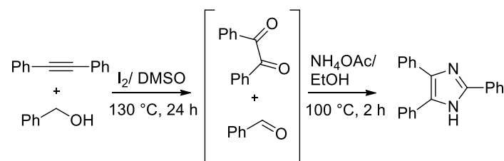
Scheme 9. Synthesis of 2,4,5- trisubstituted imidazoles.
