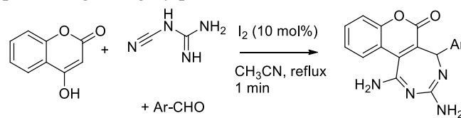
Scheme 20. The synthesis of 7-arylbenzopyrano [1,3]diazepines was catalysed by iodine.
