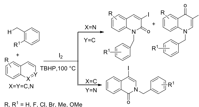
Scheme 5. The synthesis of (iodo) isoquinolinones/quinolones is described here.
