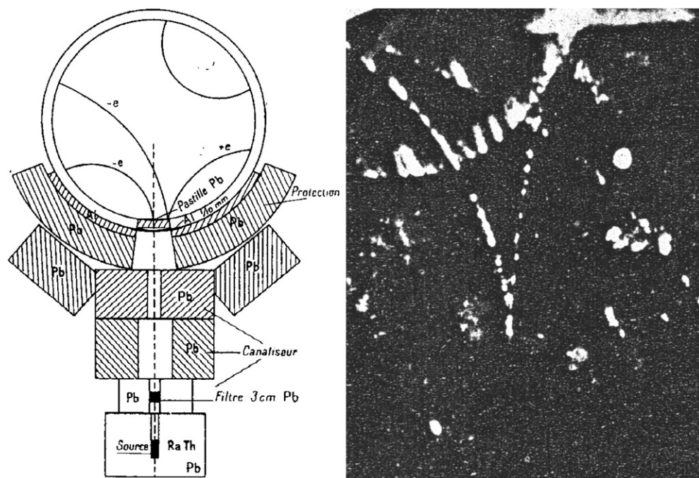
Figure 6. Schematics of Joliot–Curie apparatus for the visualization of \text{ThC}'' positrons (left) and the first Joliot–Curie’s cloud chamber photograph showing an electron–positron pair out of \gamma radiation (right) [43, table 1].
