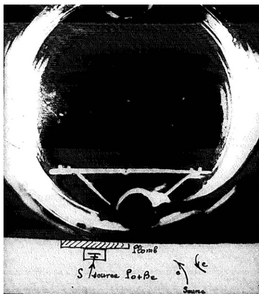
Figure 3. Photograph sent to Bohr on 26 April 1932 by Joliot and Curie [18]. This photograph is preserved by Bohr Scientific Correspondence at the Archives for History of Quantum Physics (AHQP) together with Joliot and Curie's April 26 letter (this letter is wrongly dated to August 26 in AHQP archives because of an erroneous decoding of Joliot's handwriting). Although the poor resolution of the AHQP digital image prevents a definite conclusion, in all likelihood this photograph is the same one shown in figure 1 (referred to earlier in the text) and published in Joliot and Curie's L'existence du neutron monograph [13]. As is visible in the lower side of the AHQP image, the photograph sent to Bohr, unlike the published one, was accompanied by a sketch of the behaviour of the backward electrons. From the library of the 'Accademia delle Scienze detta dei XL' in Rome, repository of Source for History of Quantum Physics.
