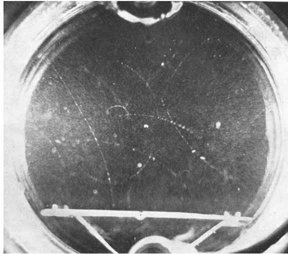
Figure 1. Joliot and Curie's photograph showing electron tracks of curvature opposite to that of others. The horizontal white band in the lower section is the paraffin screen ([16], table I).
