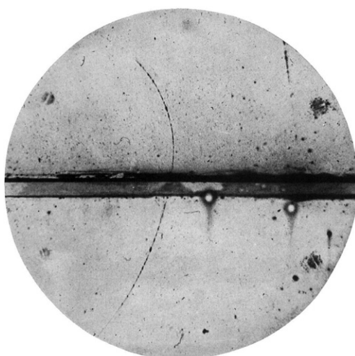
Figure 5. Anderson's cloud chamber photograph of a positron traversing the 6 mm lead plate upwards, discussed in September 1932 in Science and submitted in February 1933 to Physical Review [27]. Copyright 1933 by 'The American Physical Society'.
