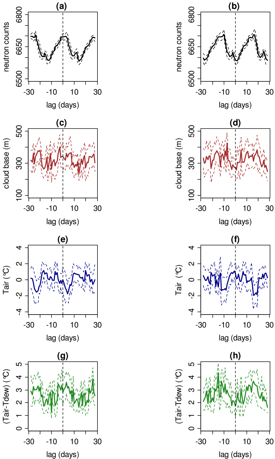
2 Figure 6. Composites formed on neutron maxima ((a), (c), (e) and (g)) and minima ((b), (d), (f) and (h)) times for (a) and (b) the neutron monitor data, (c) and (d) the Lerwick Observatory cloud base 3 height, (e) and (f) Lerwick Observatory (detrended) air temperature, (g) and (h), Lerwick Observatory 4 dew point depression from Figure 5. (Dashed lines mark 95% confidence limits on the mean values 5 obtained.) Composites are formed around the ten neutron maxima and nine neutron minima. 6
