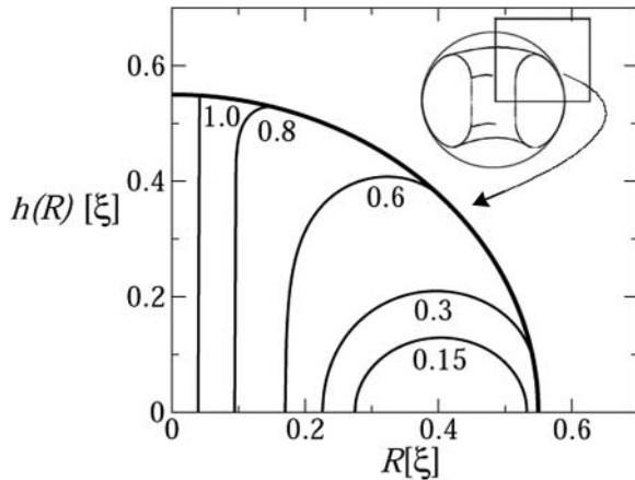
FIGURE 3 DNA packing profiles within the viral capsid. The figure shows the contour lines corresponding to the top-right quarter of the condensate's cross section, for different values of the loading fraction, L_{in}/L , as labeled.
