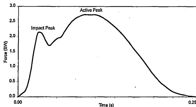
FIGURE 2—Representative vertical ground reaction force versus time curve for running.
