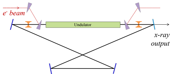
Figure 1: XFELO four crystal, two CRL cavity geometry
