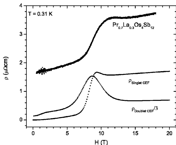
FIG. 6. Measured magnetoresistance of \text{Pr}_{0.7}\text{La}_{0.3}\text{Os}_4\text{Sb}_{12} at 310 mK for current and field along the (001) direction, and theoretical CEF resistivity for the same temperature and field direction for the singlet and doublet CEF ground states.
