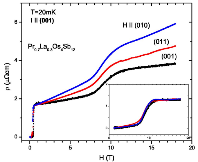
FIG. 5. (Color online) Magnetoresistance of \text{Pr}_{0.7}\text{La}_{0.3}\text{Os}_4\text{Sb}_{12} at 20 mK for three different orientations of the magnetic field. The current direction was (001). The inset shows the nearly isotropic contribution obtained by subtracting a linear (in H ) background from each isotherm.
