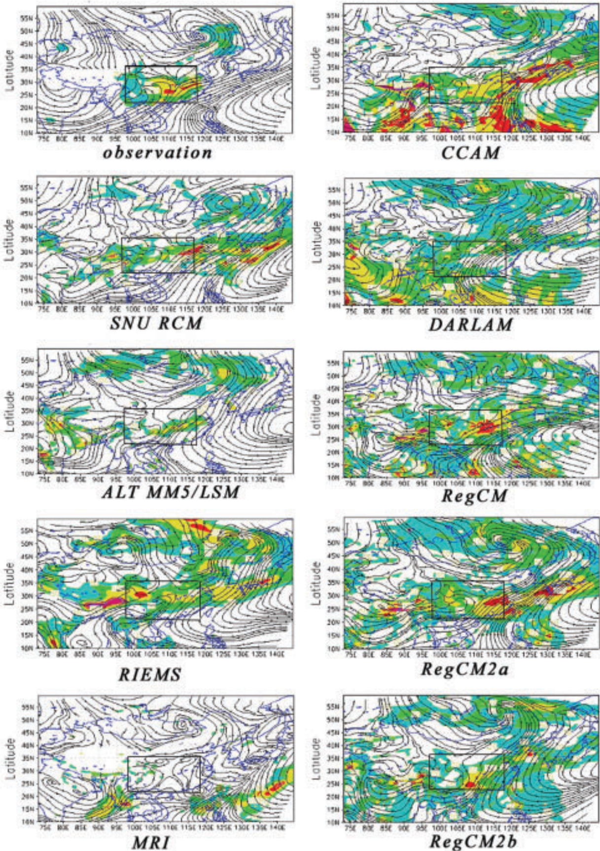
Fig. 4. Total precipitation (mm) and 850-hPa streamlines for 11–20 Jun 1998.
