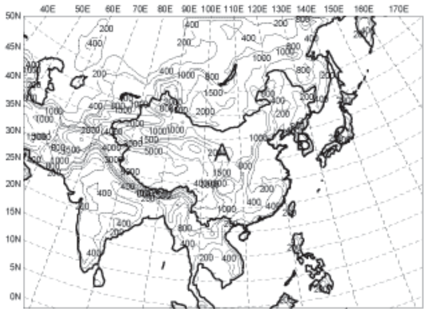
FIG. 1. MIP simulation domain, showing terrain elevations. Letters mark centers of the analysis regions: mainland China (A), Korean peninsula (B), and Japanese islands (C).
