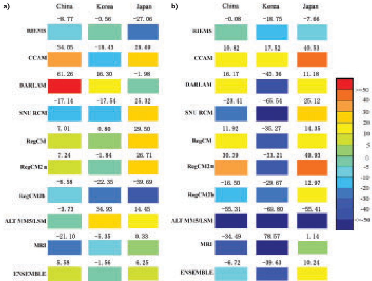
FIG. 3. Seasonal total precipitation bias (%) in (a) winter 1997 and (b) summer 1998.
