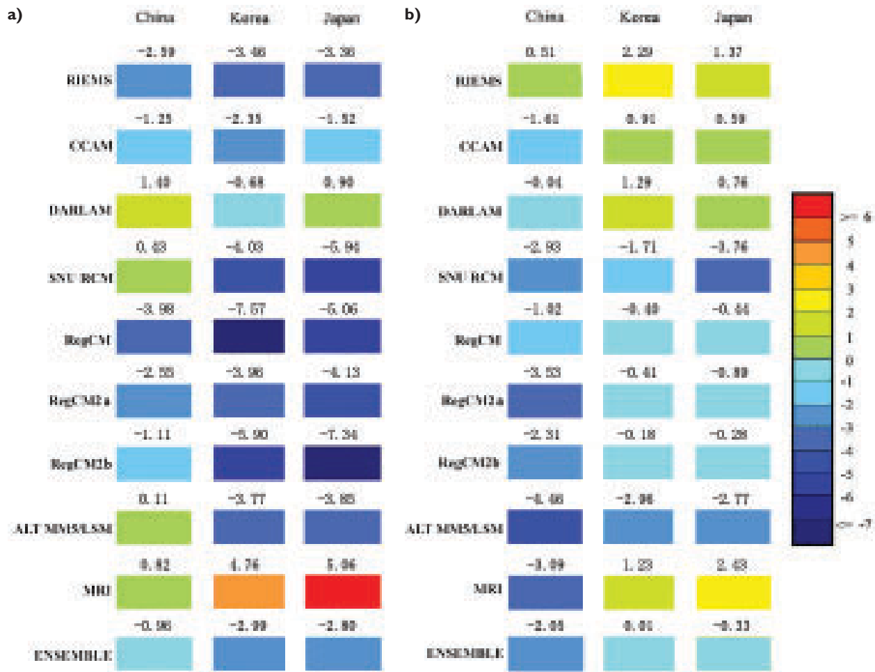
FIG. 2. Seasonal averaged surface air temperature bias ( ^{\circ}\text{C} ) in (a) winter 1997 and (b) summer 1998.
