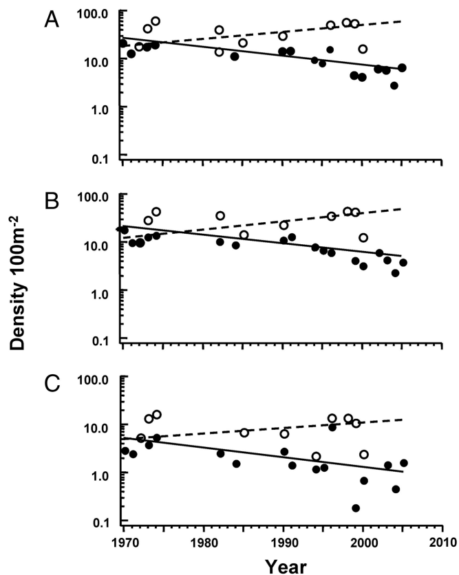
Fig. 1. Amphibian and reptile density over 35 years at La Selva Biological Station, Costa Rica. Each point indicates mean density for all quadrats in a given year. The closed symbols and solid line indicate data from primary forest. The open symbols and dashed line indicate data from abandoned cacao plantations. (A) Trends for all terrestrial amphibians and reptiles. (B) Trends for frogs only. (C) Trends for lizards only.
