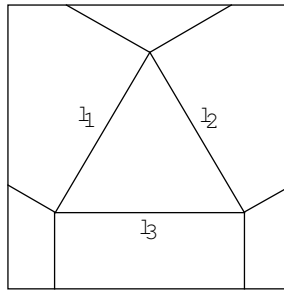
Figure 4.2: an impossible fold.
