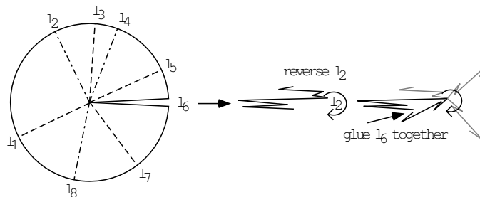
Figure 3.4: another example of how to assign creases.
