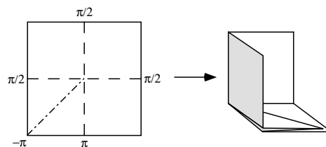
Figure 2.1: a 3-D origami.
