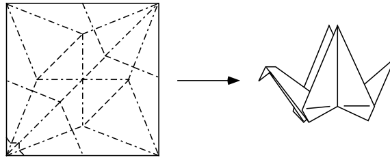
Figure 1.2: the crease-pattern for the traditional crane
