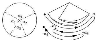
Figure 3.2: Equation (1) in action.
