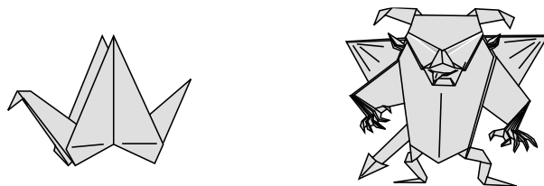
Figure 1.1: two origamis folded from single, uncut squares, the traditional crane and Jun Maekawa's winged demon.
