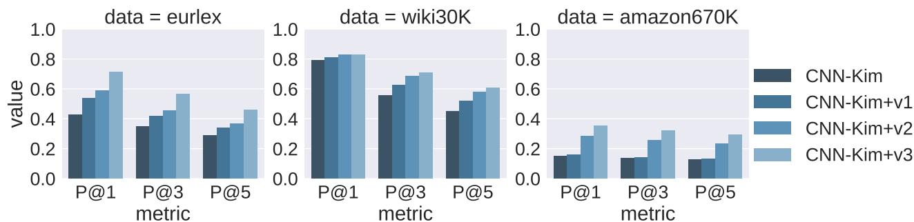
Figure 2: Result of the ablation test – v1 uses the new loss function for multi-label classification over CNN-Kim; v2 denotes the insertion of the additional hidden layers over v1, and v3 denotes the insertion of the dynamic max pooling layer over v2 (hence the full version of XML-CNN).
