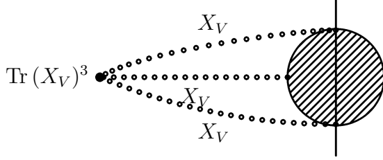
Figure 2: The generic contribution to the one point function \langle \text{Tr}(X_V)^k \rangle with all k X_V lines pinned to the defect (vertical line), depicted here for k = 3 .
