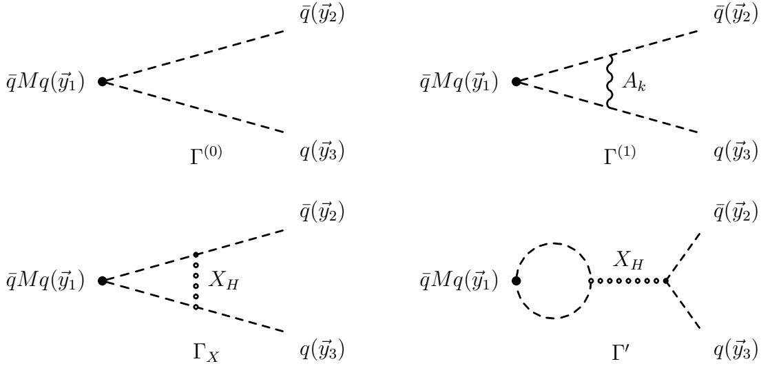
Figure 1: Feynman diagrams through one-loop order for the correlators \langle \bar{q} M q(\vec{y}_1) \bar{q}(\vec{y}_2) q(\vec{y}_3) \rangle where M is either \sigma^A or 1.
