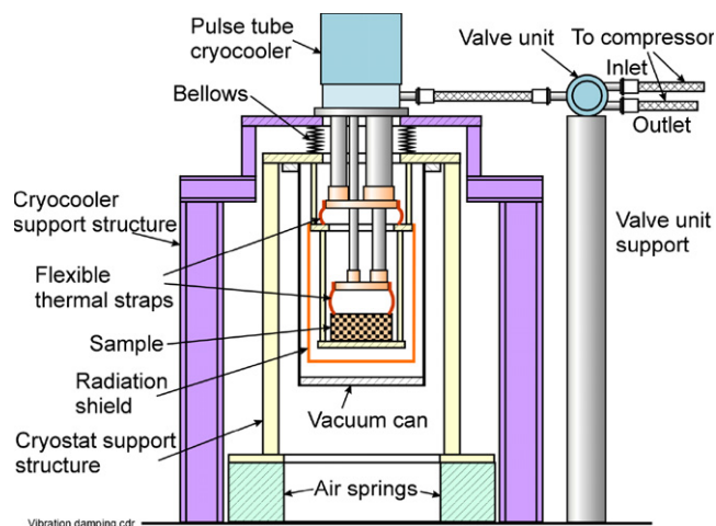
Figure 5. Cryocooler vibration damping scheme capable of achieving 0.1 \mu\text{m} vibration amplitudes.
