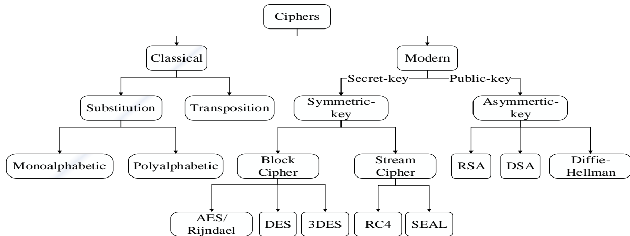
Fig 1: Classification of Encryption Methods
