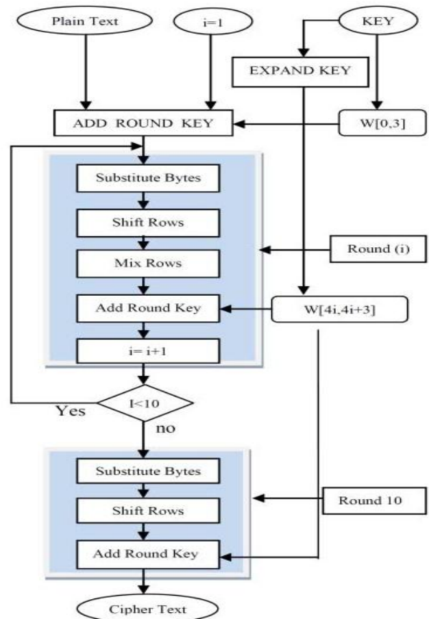
Fig 4: AES (Advanced Encryption Standard) process [10]
