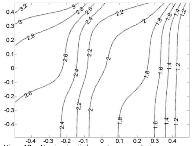
Fig. 12. Equipotential contours – heterogeneous medium, structured mesh 2 nd refinement level (dashed lines: MHFE and MMHFE methods, dotted lines FV2 method)
