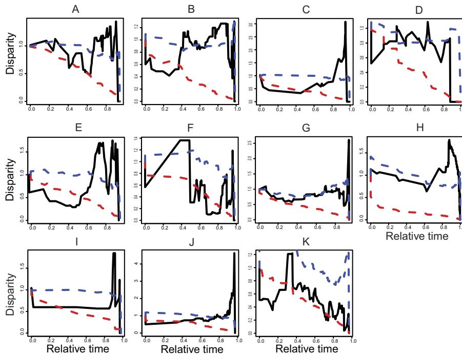
Figure 2. Disparity through time in extinction risk. (A) Cypereae, (B) Disa , (C) Indigofera , (D) Lachnaea , (E) Muraltia , (F) Pentaschistis , (G) Podalyriaceae , (H) Restionaceae, (I) Zygophyllum , (J) Protea , and (K) Moraea . Solid line, observed values; dashed red line, Brownian expectations; dashed blue line, punctuated model (range asymmetry factor = 2, s.d. for evolutionary drift = 2, evolutionary trend = 0.3; Materials and Methods). Clade age is scaled between 0 and 1, with 0 zero representing clade origins and 1 representing the present day. High relative disparity towards the present (e.g., Cypereae, Indigofera , Muraltia , Podalyriaceae , Protea , and Restionaceae) indicates that most variation in extinction risk is between species within subclades, i.e. closely related species frequently differ strongly in extinction risk. Low relative disparity towards the root of the tree (e.g., Disa , Indigofera , Moraea , and Muraltia ) indicates that most variation in extinction risk is between subclades, i.e. species are more similar in extinction risk within subclades than between subclades. doi:10.1371/journal.pbio.1000620.g002
