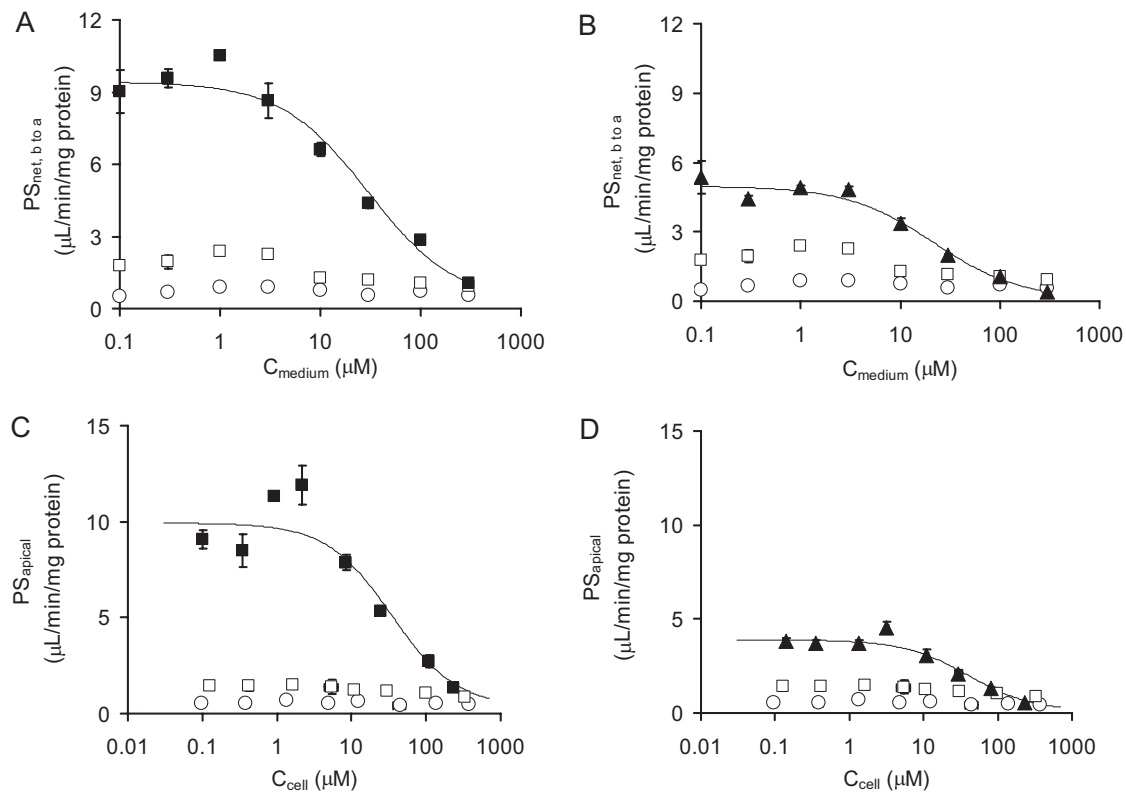
FIG. 4. Concentration dependence of the transcellular transport clearance ( PS_{net} ) (A and B) and apical transmembrane clearance ( PS_{apical} ) (C and D) of rosuvastatin across MDCKII monolayers expressing OATP1B1/MRP2 (A and C) or OATP1B1/MDR1 (B and D). The concentration dependence of PS_{net} from the basal to the apical side (A and B) and of PS_{apical} (C and D) across MDCKII monolayers expressing both OATP1B1 and MRP2 (■) or both OATP1B1 and MDR1 (▲) were compared with those across an OATP1B1-expressing monolayer (□) or a vector-transfected control MDCKII monolayer (○). PS_{net} from the basal to the apical side and PS_{apical} for 120 min were determined at various concentrations of rosuvastatin (0.1–300 \mu M). The data were fitted to eq. 6 (described under Materials and Methods ) by the nonlinear least-squares method, and each solid line represents the fitted curve. Each point represents the mean \pm S.E. ( n = 3 ). Where vertical and/or horizontal bars are not shown, the S.E. values are within the limits of the symbols.
