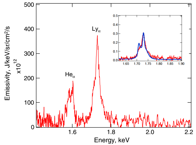
FIG. 3 (color online). X-ray emission spectra from shock compressed aluminum in diamond. Inset comparison of measured and simulated Ly_\alpha line shape indicates 9 g/cc.
