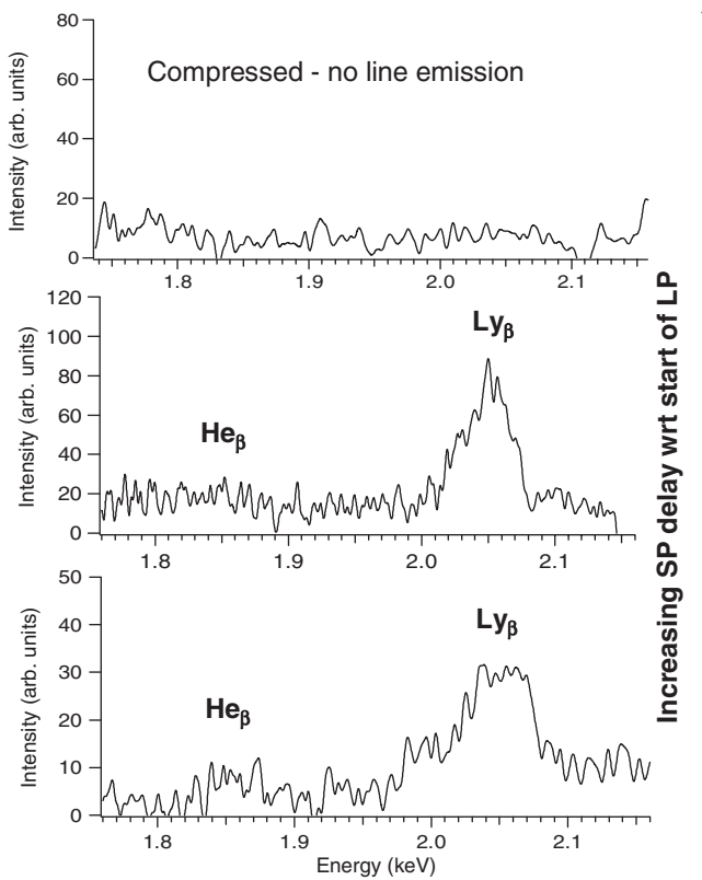
FIG. 2. Emission spectra recorded on the streak camera at various times during the shock wave transit through the target. For the bottom and middle curves the shock has not yet arrived at the aluminum layer position. In the top curve the shock has compressed the aluminum and the n = 3 levels have become delocalized.
