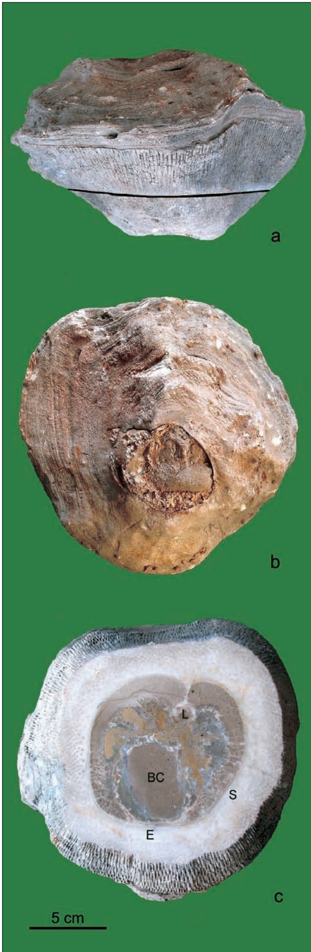
Fig. 2 a. Pseudopolyconites slovenicus n.sp. – upper and lower valve; holotype; Gorica Museum: Museal exposition of Stanislava Bačar's fossils at Ajdovščina, sample no. 8142, Bitež near Grgar.
