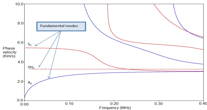
Fig. 8: Dispersion curves for a steel plate of 1.5 mm thickness
