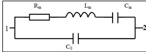
Fig. 3: Illustration of the electronic equivalent circuit model of a common piezoelectric transducer. C_0 is the electrical capacitance of the transducer and L_m , C_m , and R_m describe the resonance mechanical properties of the transducer.
