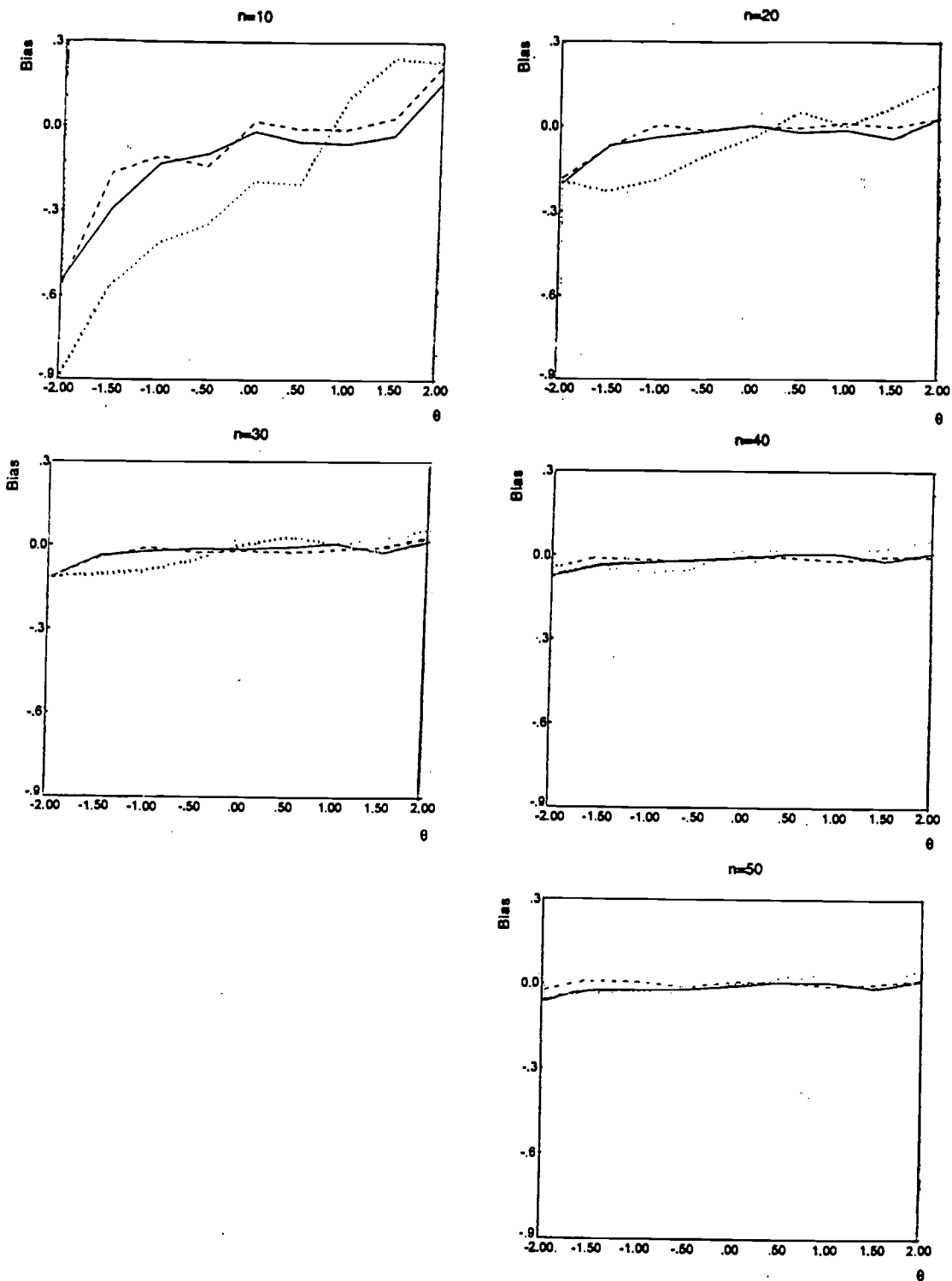
FIGURE 2. Estimated bias functions of the EAP estimator of ability after 10, 20, 30, 40, and 50 items (solid line: unconstrained CAT; dashed line: constrained CAT, in the order IA, SA, SB; dotted line: constrained CAT, in the order SA, SB, IA).
