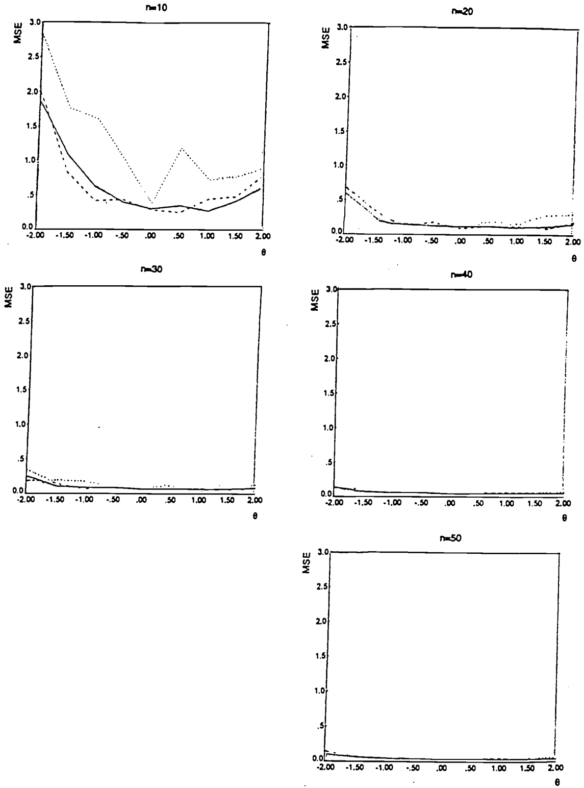
FIGURE 1. Estimated MSE functions of the EAP estimator after 10, 20, 30, 40, and 50 items (solid line: unconstrained CAT; dashed line: constrained CAT, in the order IA, SA, SB; dotted line: constrained CAT, in the order SA, SB, IA).
