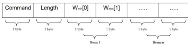
Fig. 3 GA_CHROMOSOME packets
