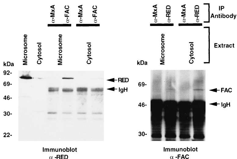
Fig 2. Detection of murine fac-RED complexes in liver extracts. Using the indicated antibodies and protein A-agarose, mouse liver cytosolic or microsomal extracts (730 \mu g) were used to immunoprecipitate fac, and immune complexes were analyzed for the presence of RED by probing the immunoblot with anti-RED antibodies (left). Each subcellular fraction (50- \mu g aliquots) was also analyzed directly without prior IP. Conversely, immune complexes obtained by IP with anti-RED antibodies were analyzed for the presence of FAC by immunoblotting (right). After SDS-PAGE (10% gel for the left panel, 8% to 20% gradient gel for the right panel), immunoblots were probed with the antibodies indicated in the bottom of the figure.
