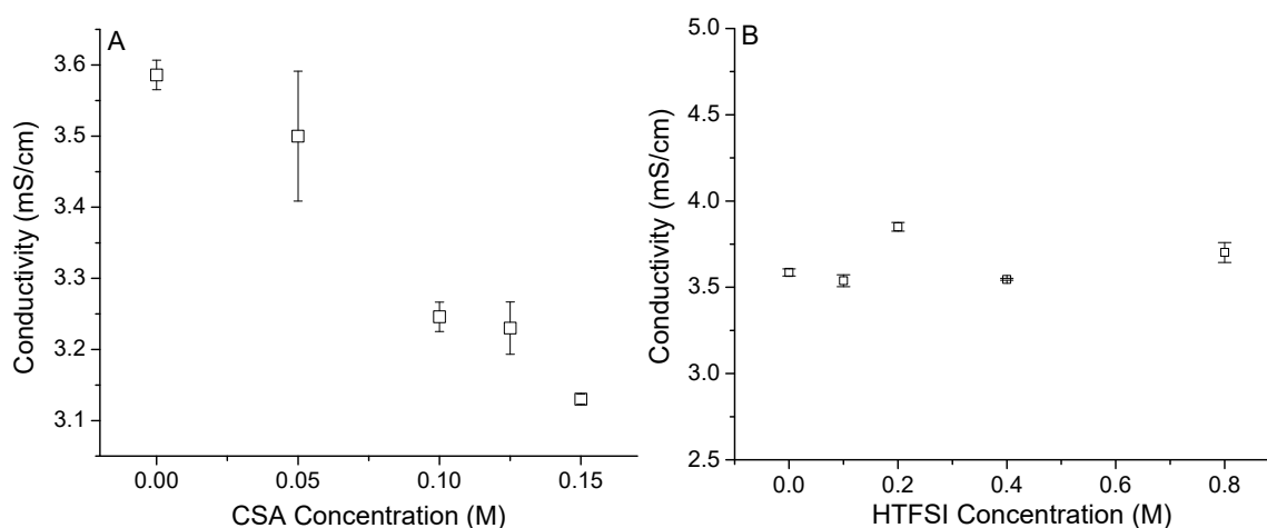
Figure 10. Conductivity of CSA solutions in BMIBF 4 (A) and HTFSI solutions in BMIBF 4 (B).
