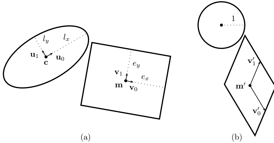
Figure 1. (a) Illustration in 2D showing the representation used for the ellipsoid and the OBB. (b) The corresponding illustration in 2D of the resulting sphere and parallelepiped shapes after the transformation of space. The parameters of the parallelepiped are computed according to Equations (2)–(5).
