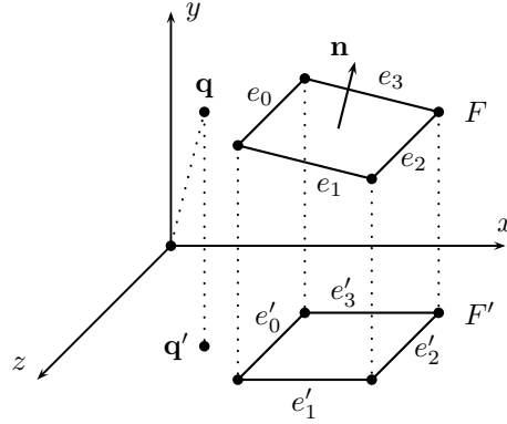
Figure 3. To determine the distance from the origin to the polygon F with edges e_i , a combination of calculations in 2D and 3D is used. Projections are shown with dotted lines.
