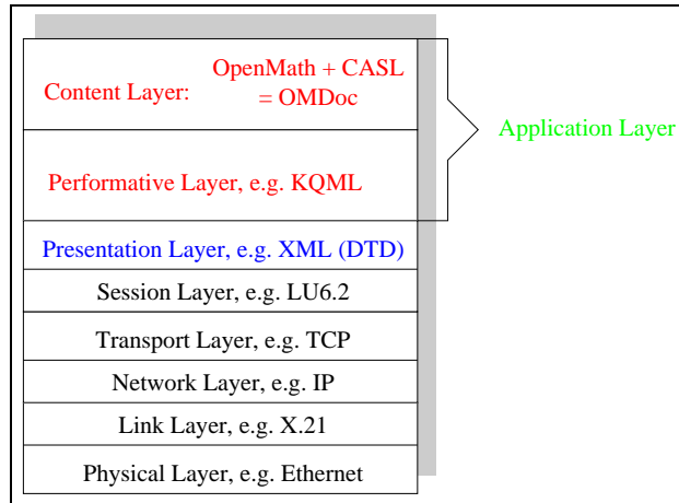
Fig. 1. Artificial Communication: KQML and the OSI Reference Model
