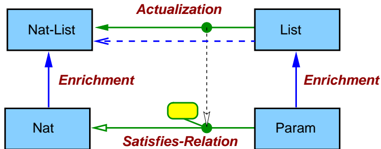
Fig. 6. A Structured Specification of Lists
