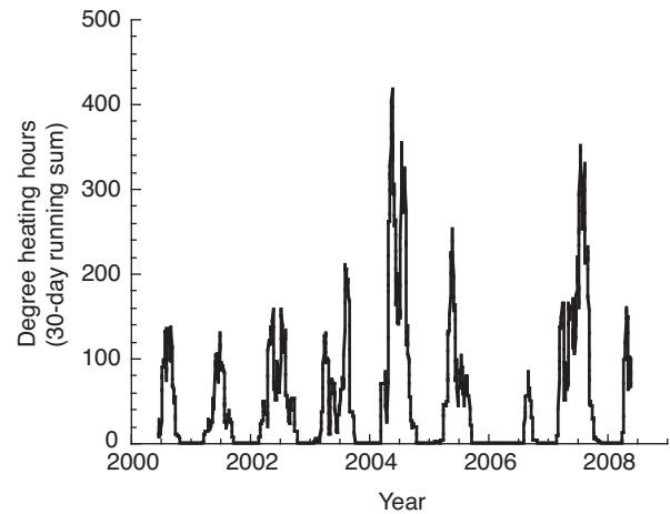
Fig. 4. Estimation of degree heating hours at the Hopkins Marine Station (Pacific Grove, CA, USA) intertidal site. Values were calculated by adding the degree hours above a threshold of 25°C (the observed peak mean daily temperature at this site) using a running sum of 30 days.
