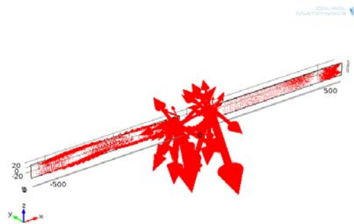
Figure 5. The SI Map of Bolt Joints Structure at Tightening Torque =2Nm
