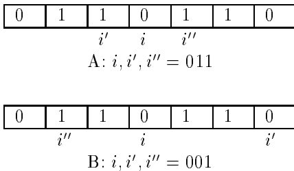
Figure 4: At the top, gene i is linked to neighbours i' , i'' . The values 011 point into a fitness look-up table for i . Below, i' and i'' are no longer immediate neighbours.
