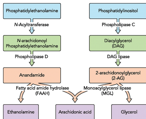
Fig. 1. Synthesis and degradation of 2-arachidonoylglycerol and anandamide. (Adapted from El Manira and Kyriakatos 2010, with permission of Physiology , Vol. 25, p. 231, © 2010 The American Physiological Society.)
