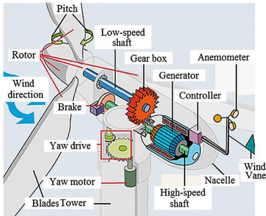
Figure 1. Internal Structure of Wind Turbine [8]
