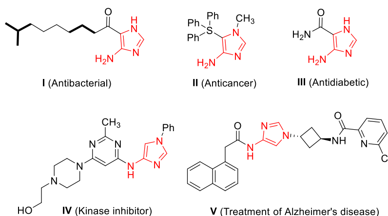
Figure 1. Selected drug molecules containing the 4-aminoimidazole moiety.
