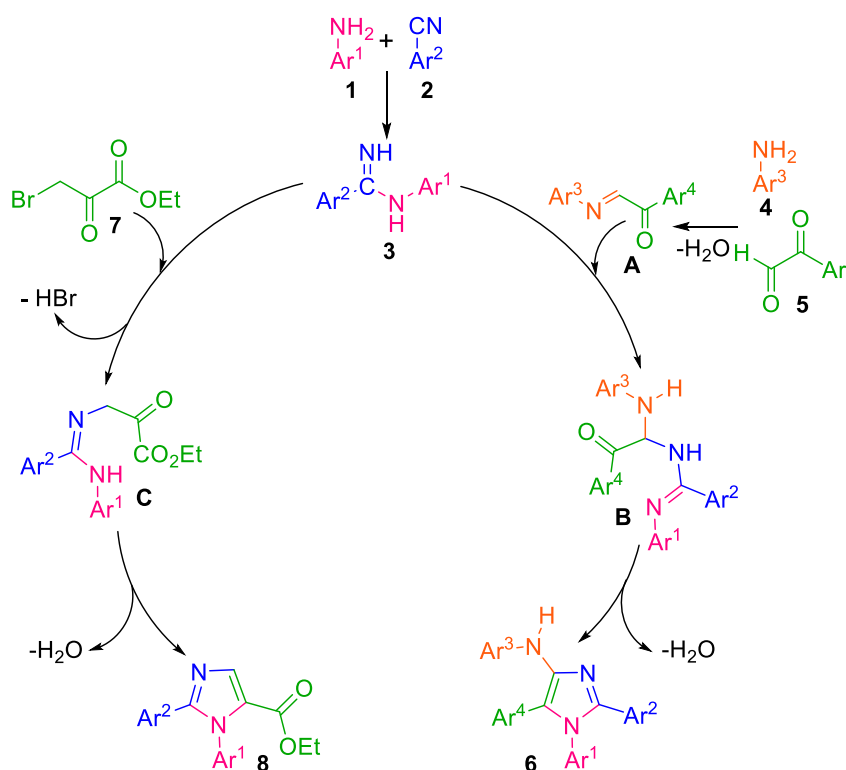
Scheme 1. Proposed mechanism for the synthesis of 4-amino-1,2,5-tetrasubstituted imidazoles 6 , and 1,2,5-trisubstituted imidazoles 8 .
