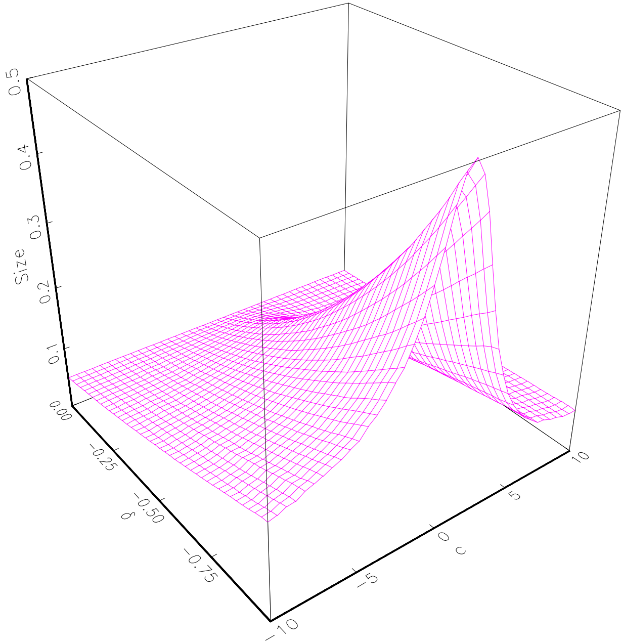
Figure 4: Asymptotic Size of One-Sided t -test at 5% Significance
