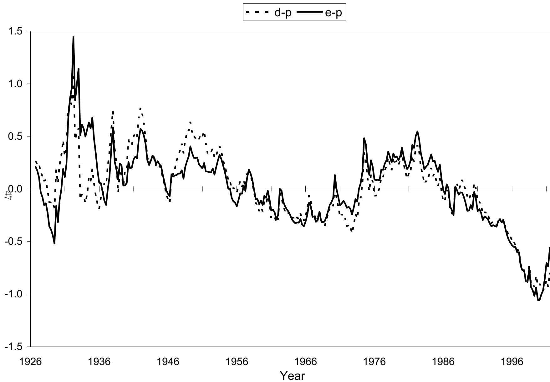
Figure 2: Time Series Plot of Valuation Ratios
