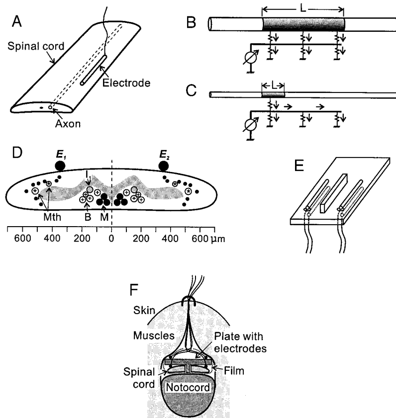
FIG. 1. Macroelectrodes for recording activity of reticulospinal (RS) axons. A : orientation of the an electrode on the dorsal surface of the spinal cord in relation to the position of the RS axon. B and C : wire electrode serves as a filter for recording spikes almost exclusively from the larger fibers. Length of the electrode (3 mm) was approximately equal to the longitudinal extent of the axonal membrane excited by the propagating spike ( L ) in the thicker RS axons ( B ). For the thinner axons, L was smaller and the efficiency of recording was reduced because of shunting ( C ). Arrows in B and C indicate extraaxonal currents. D : position of the electrodes ( E_1 and E_2 ) in relation to the spinal cord. Location of the large-size RS axons of Mauthner cells (Mth), Müller cells (B, M, and I types), and middle-size axons (small black circles) on the cross-section of the spinal cord is shown schematically. E : design of electrodes, view from below. Four silver wires (75 \mu\text{m} diam and 3 mm length) were glued to a plastic plate with a longitudinal wall. F : position of the implanted plate with electrodes as seen on the transversal section of the lamprey's body. Plate with the electrodes together with the adjoining segments of the spinal cord were isolated electrically from the surrounding muscles by a strip of thin (20 \mu\text{m} ) plastic film.
