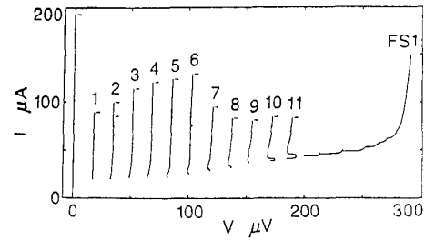
Figure 2. Typical recorded dc IV -characteristic (sample H5-2A, \ell = 5.5 mm, w = 200 \mu m) showing the first mode step, MS1 and a series of parametrically generated mode steps, PMS k . The temperature was 4.2 K and an external magnetic field, B = 272 \mu T was applied. The arrows indicate the current at which the junction switches from the step. The structure to the right is the first Fiske step at 295 \mu V. The position of the foot-like structures visible on higher numbered PMS k agree with the voltages of the corresponding mode steps, MS n .
