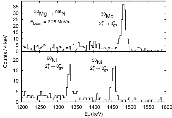
FIG. 1: Doppler-corrected \gamma -ray spectra observed in coincidence with projectiles in the CD detector. The upper panel shows the spectrum performing a Doppler correction relevant for \gamma emission from the detected projectile (without Ni-line contributions, see text), while the Doppler-corrected spectrum assuming \gamma emission from the corresponding recoiling target nucleus is displayed in the lower panel (without the Mg-line contributions, see text).
