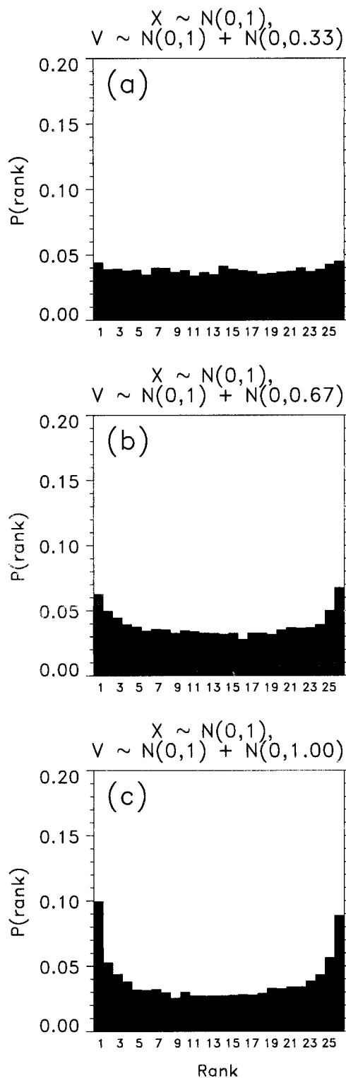
FIG. 6. Rank histograms in presence of observational error. Ensemble sampled from N(0, 1) distribution, observation from N(0, 1) + N(0, \sigma) distribution. Verification rank tallied 10 000 times. (a) \sigma = 0.33 , (b) \sigma = 0.67 , (c) \sigma = 1.00 .
