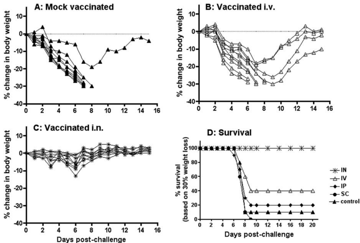
Figure 2. Intranasal vaccination with \gamma -Flu provides superior protection to heterotypic virus challenge. Groups of 10 BALB/c mice were either mock treated (A) or vaccinated with \gamma -A/PC ( 3.2 \times 10^6 PFU equivalents) intravenously (B) or intranasally (C). Mice were challenged intranasally after 3 weeks with a lethal dose ( 6 \times 10^2 PFU) of A/PR8 and weight recorded daily for 21 days. Survival (D) of mice mock treated, or vaccinated i.n., i.v., i.p., or s.c. and challenged as for (A–C) and monitored for 21 days. doi:10.1371/journal.pone.0005336.g002
