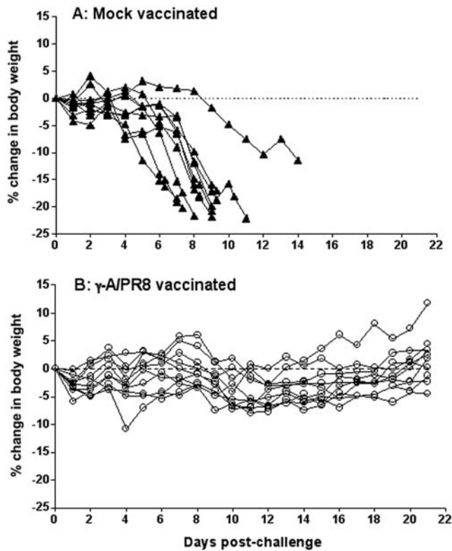
Figure 3. Intranasal vaccination with \gamma -Flu ( \gamma -A/PR8(H1N1)) protects against H5N1 challenge. Groups of 10 BALB/c mice were either mock treated (A) or vaccinated with \gamma -A/PR8 (B). Mice were challenged 4 weeks later with 3 MID 50 of A/Vietnam/1203/2004[H5N1] intranasally and weight recorded daily for 21 days. doi:10.1371/journal.pone.0005336.g003
