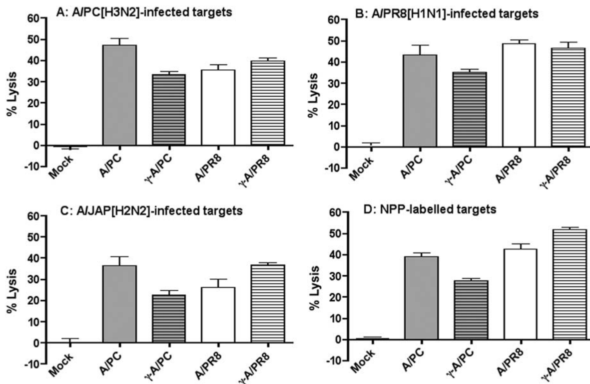
Figure 1. Cross-reactive cytotoxic T cell responses induced by \gamma -Flu. 10-week-old BALB/c mice were either infected or vaccinated with live A/PR8, \gamma -A/PR8, live A/PC, or \gamma -A/PC. Six days later, splenocytes from these mice were tested for their killing activity against mock, A/PC-, A/PR8-, A/JAP-infected, and NPP-labelled P815 targets. Data represent % specific lysis after 6 h assay time at an effector to target cell ratio of 120:1. doi:10.1371/journal.pone.0005336.g001
